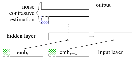
Figure 5: Choice for RNN-LM enhancement, hatched. Either as input (bottom, ) or in NCE (top, ) .
