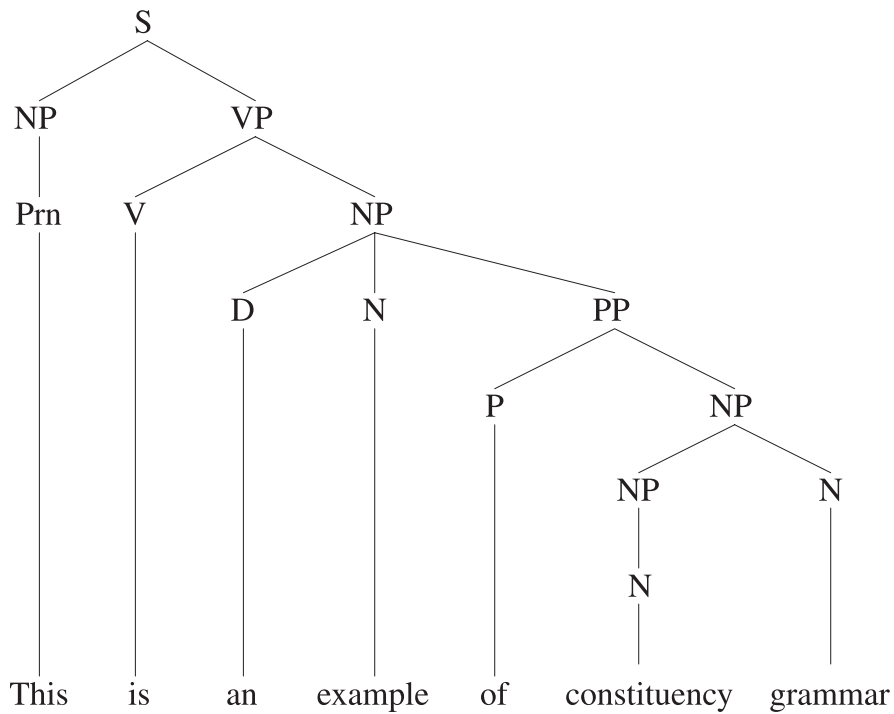
Figure 1: A constituency tree.
