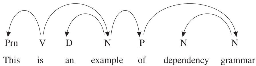
Figure 2: A dependency tree is a set of links connecting heads to dependents.
