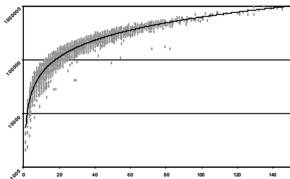
Instructions / number of words for Shallow Parser (logarithmic scale)
